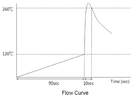
Flow Curve
