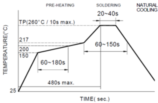
Re-flow Soldering(Lead Free)
