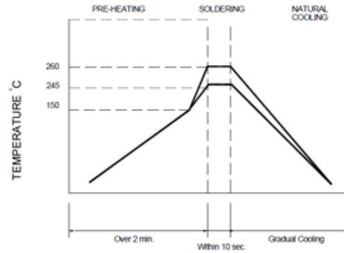
Wave Soldering
