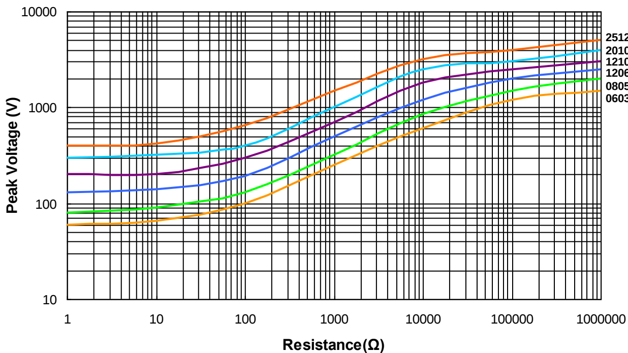
SWR Series 10/700us Lightning Surge
